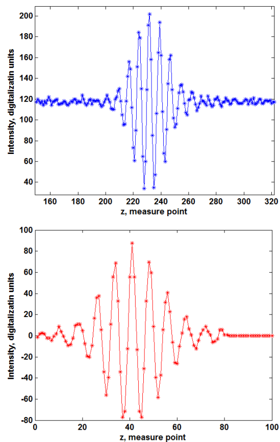
Figure 3. A typical correlogram measured on smooth surface (picture above) and the correlogram used as the reference correlogram (below).
