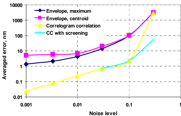
Figure 2. Mean deviation obtained by the two envelope methods and the correlogram correlation method.
