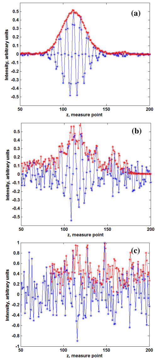
Figure 1. Correlogram corruption at different noise levels: (a) – noise dispersion \sigma_{noise} is 0.01 of the double correlogram amplitude; (b) \sigma_{noise} = 0.1 ; (c) \sigma_{noise} = 0.3 . The red lines show the corresponding envelope.
