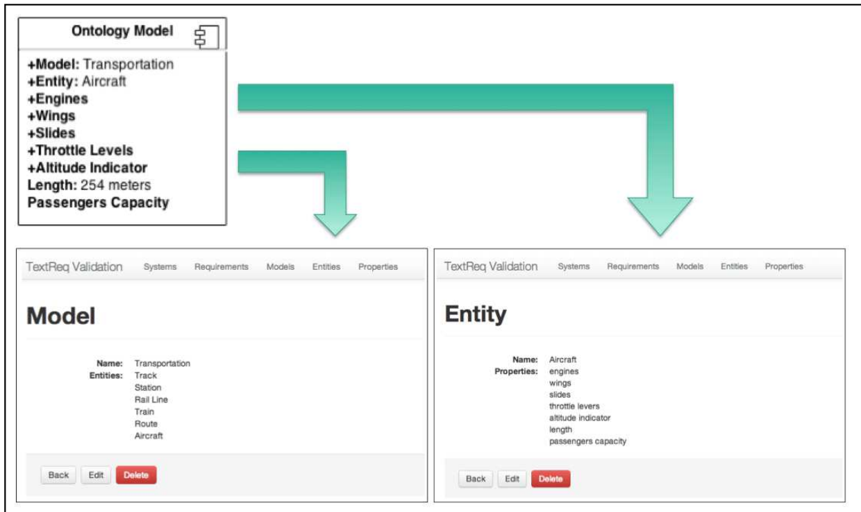
Figure 11. Relationship among aircraft and transportation ontology models, and an aircraft entity model. Top left: Simplified ontology model for an aircraft. Bottom left: Detailed view of the Transportation ontology model. Bottom right: Detailed view for the entity Aircraft.
