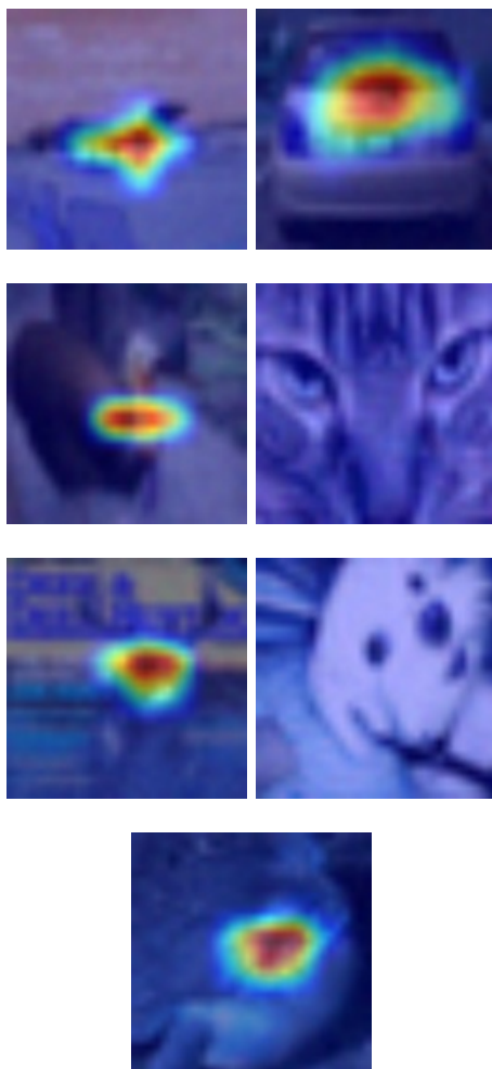
Fig. 5. Illustration of attention shift using Grad-CAM on model trained by AICR loss. Adversarial images are obtained crafted with PGD ( \epsilon = 0.03 ); compare with clean images in Figure 4.
