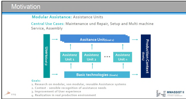
Figure 3. MMAstist_II Motivation
