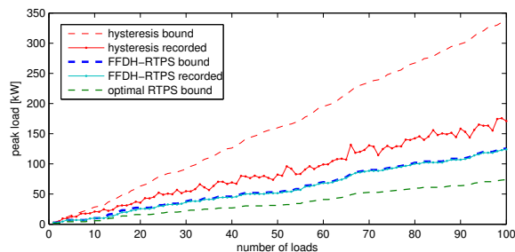
Fig. 5. Comparison between hysteresis- and RTPS-control methods. The RTPS-controlled actual behavior, during the simulation of 120 hours, reduces the peak load of the 35% in respect of hysteresis control in regular working conditions. The improvement on the theoretical bound associated with worst case working conditions is around 60%.
