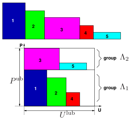
Fig. 3. Example of level packing using the FFDH algorithm. Five items are firstly ordered by non-increasing height and then packed into two levels. Note that item 3 generates a new level \Lambda_2 since it does not fit at the right of item 2 within level \Lambda_1 . The load utilizations of the 5 loads are respectively (0.28, 0.26, 0.49, 0.22, 0.30). Their consumed power are (5, 4, 3, 2, 1). The schedule generated by this system is depicted in Fig. 1.
