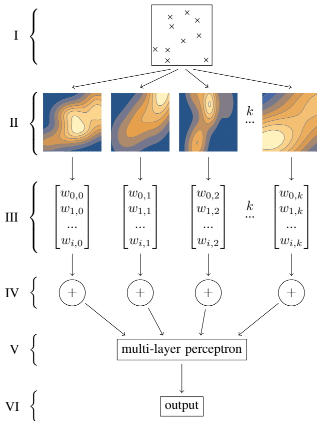
Fig. 1. Overview of a continuous feature network.
