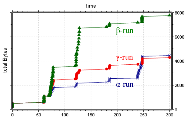
Figure 9. Total size of processed LISP control messages by xTR1
