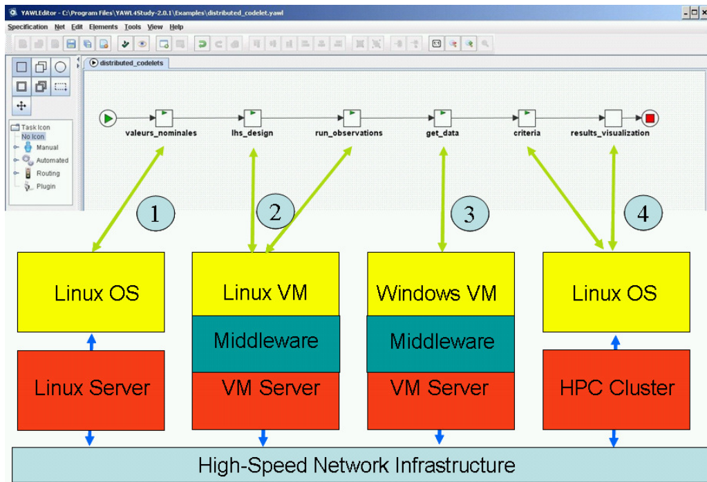
Figure 20. The distributed simulation platform.
