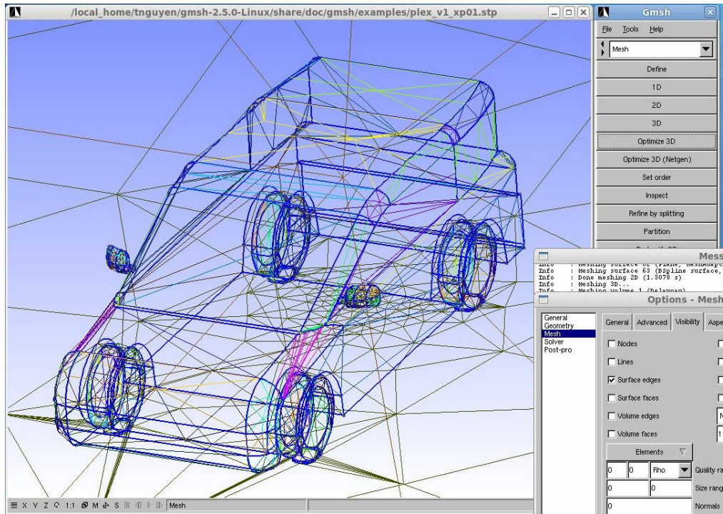
Figure 21. Mesh for vehicle aerodynamics simulation (Gmsh screenshot).
