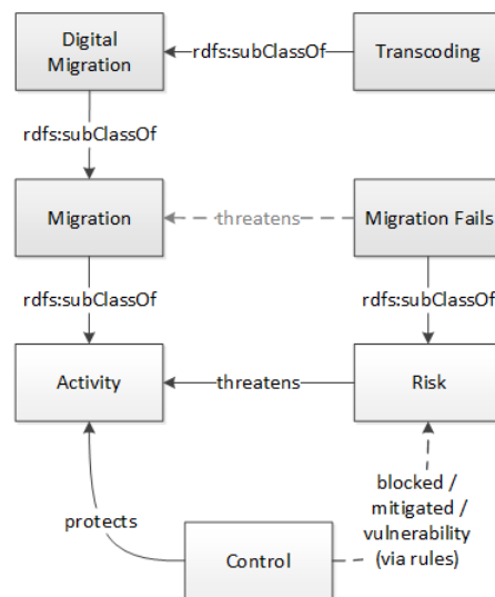
Figure 6. BPRisk ontology with sub-classing examples. CORE layer entities depicted in white and DOMAIN layer entities in grey.
