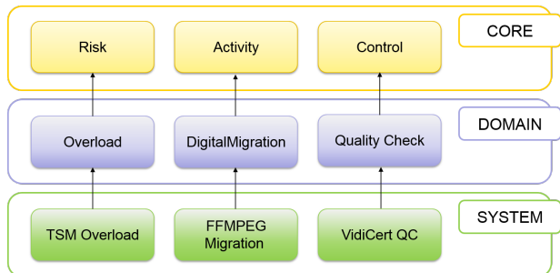
Figure 5. Workflow risk ontology layers.
