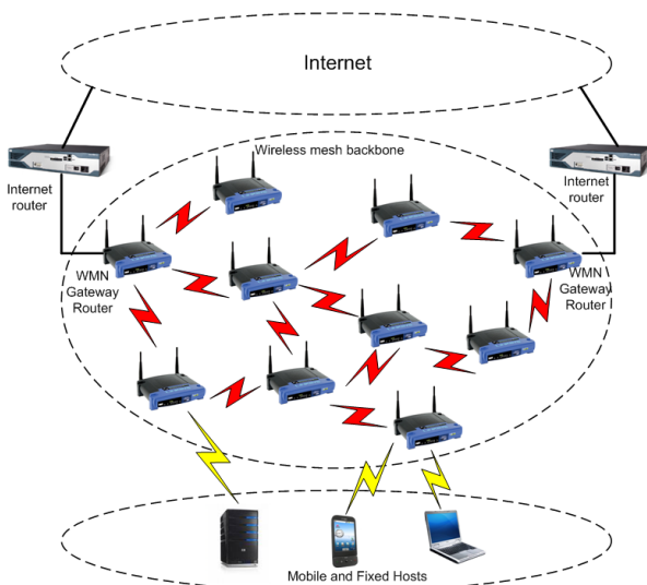
Figure 1. Diagram of a Wireless Mesh Network
