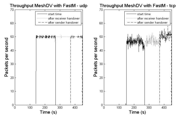
Figure 7. Throughput of MeshDV with FastM in the static case and in case of handover (receiver at t=270 s, sender at t=370 s).
