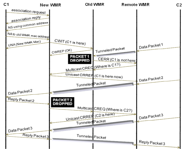
Figure 2. Communication diagram of EMM
