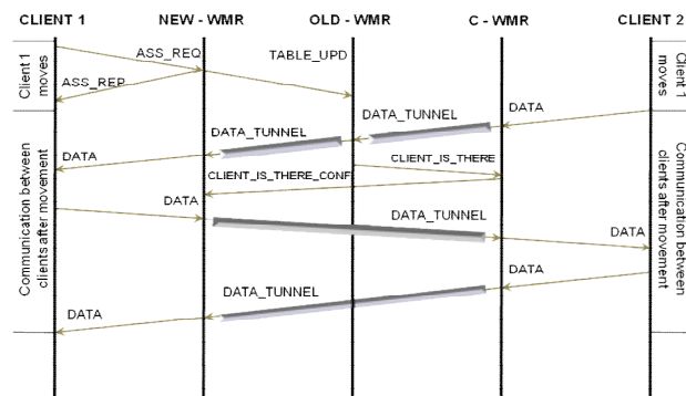
Figure 3. Communication diagram of FastM
