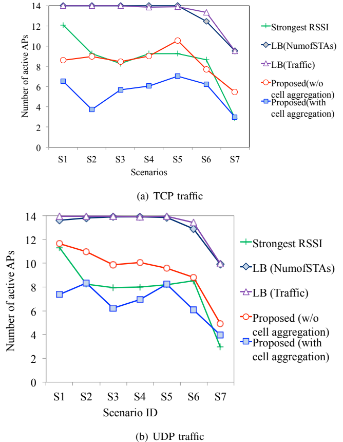
Figure 8. Comparing the number of active APs for each scheme. The figures show that the load balancing schemes tend to use all the existing APs. The proposed scheme without cell aggregation utilizes around the same number of APs as that of Strongest RSSI scheme. The proposed scheme with cell aggregation utilizes the smallest number of APs.
