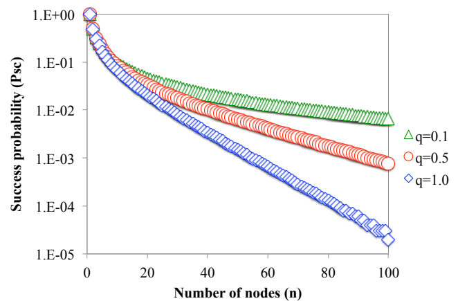
Figure 2. Success probability as a function of the number of contending nodes. The figure shows that P_{sc} sharply decreases with the increase of the number of nodes. The smaller the probability of having a pending frame ( q ), the larger is the P_{sc} .
