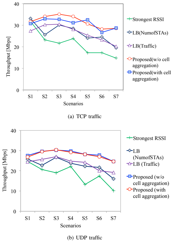
Figure 7. Comparing throughput performance for TCP and UDP traffic. The figures show that Strongest RSSI scheme is inferior to the remaining schemes and the proposed scheme shows the best performance.
