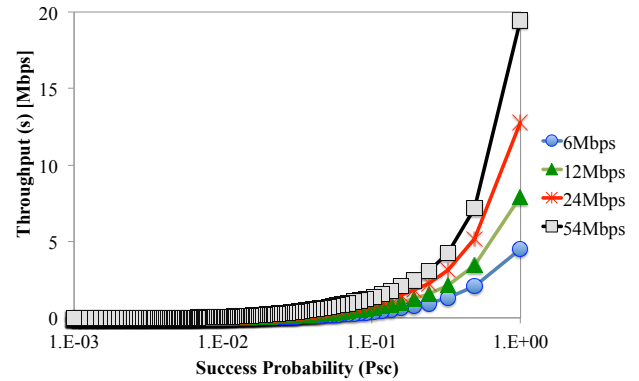
Figure 4. The throughput performance as a function of the success probability. The figure shows that for a sufficient throughput is achieved only when the success probability is large.
