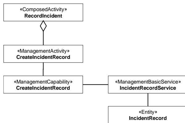
Figure 7. Domain Model for IncidentRecordService
