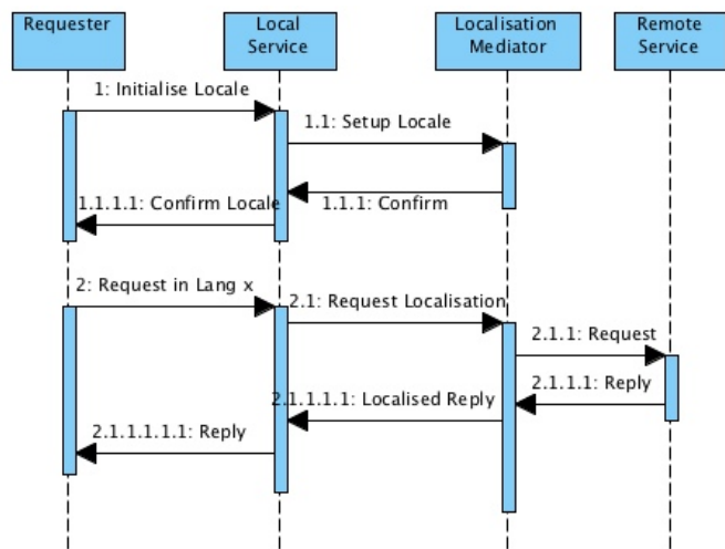
Fig. 3: A UML Sequence Diagram of the Platform.
