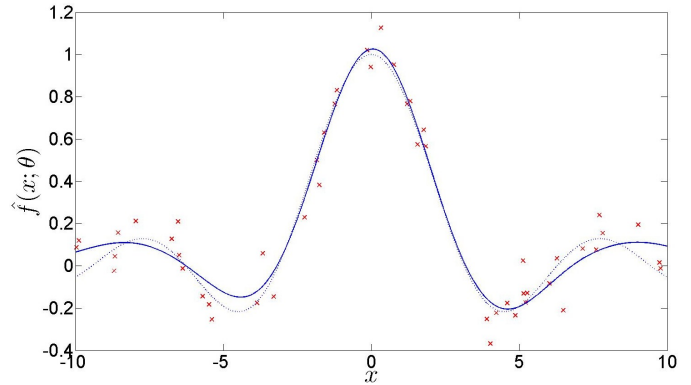
Fig. 2. Typical regression.
