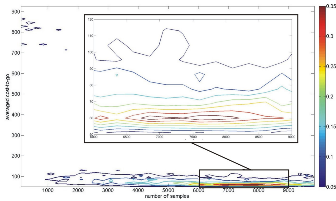
Fig. 9. Mountain car.
