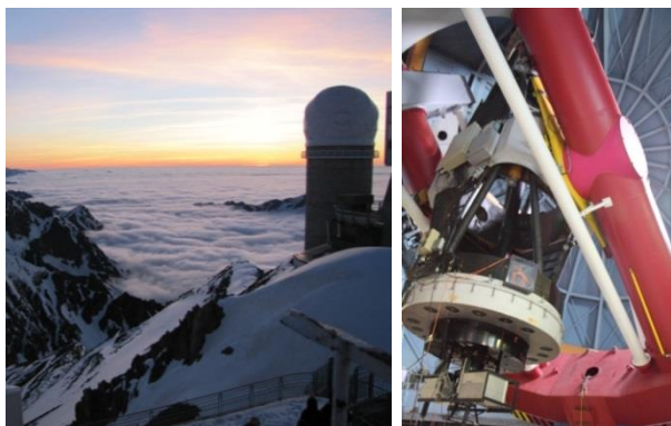
Figure 2. The Telescope Bernard-Lyot outside (left) and inside (right).
